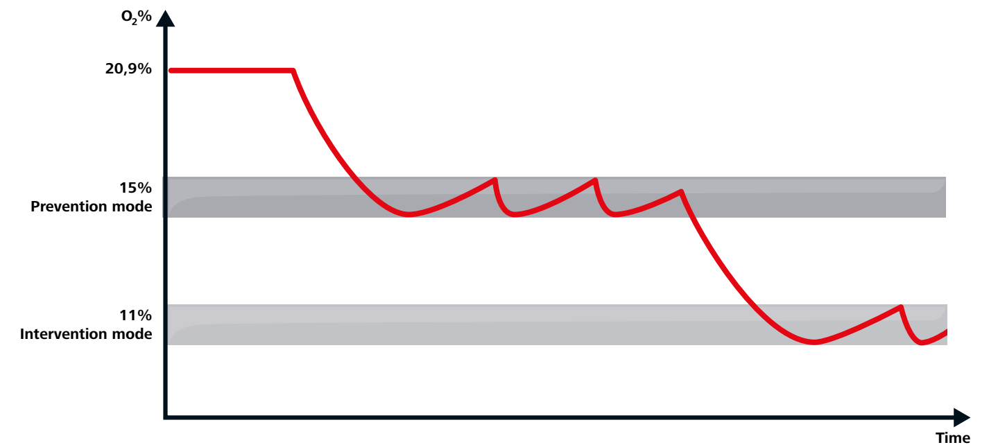
Figure 12: Control curve of the Oxeo EcoPrevent CS with prevention mode and intervention mode
