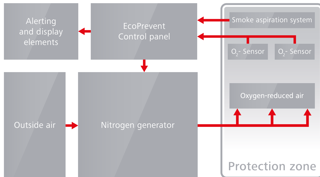
Figure 3: Process schematic of a Minimax oxygen reduction system
