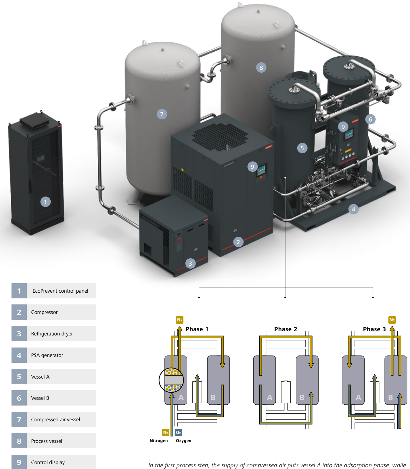
Figure 8: Design of the Oxeo EcoPrevent PG
