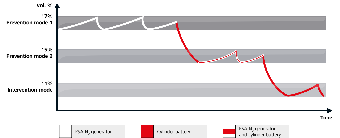
Figure 14: Control curve of the Oxexo EcoPrevent PG/CS hybrid solution
