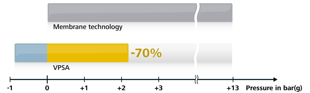
Figure 10: Comparison of the process pressure of membrane vs. VPSA technology
