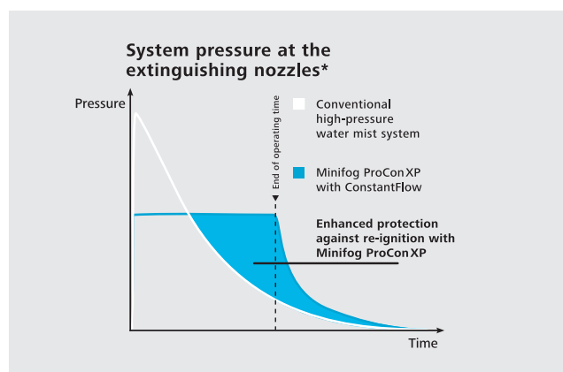
System pressure at the nozzles *
